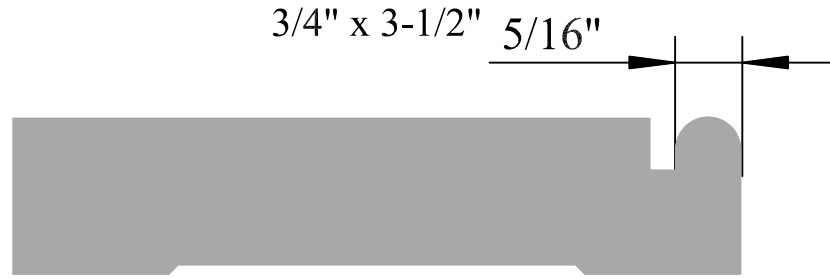
FL # 129 3/4"x 3-1/2"-9-1/4"
