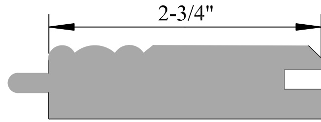
FL # 143 3/4"x 2-3/4"
