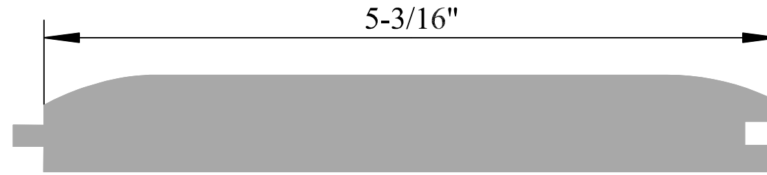
FL # 459 3/4" x 5-3/16"
