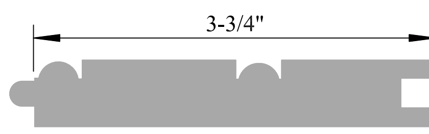
FL # 496 5/8"x 3-3/4"
