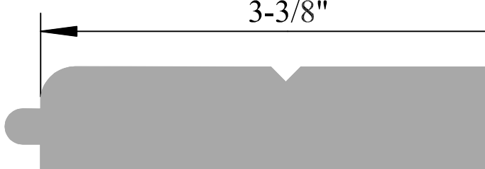
FL # 386 3/4"x 3-3/8"
