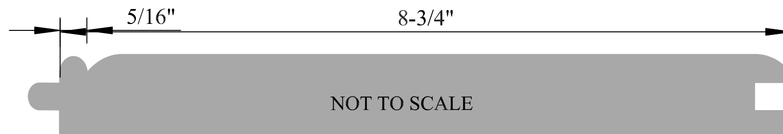
FL # 217 1"x 10"
