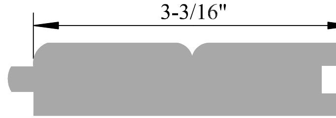
FL # 250 3/4"x 3-3/16"
