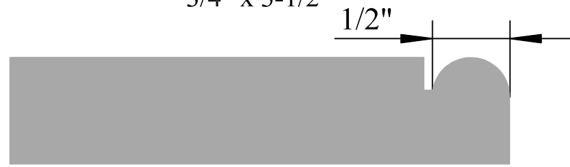
FL # 214 3/4" x 3-1/2"
