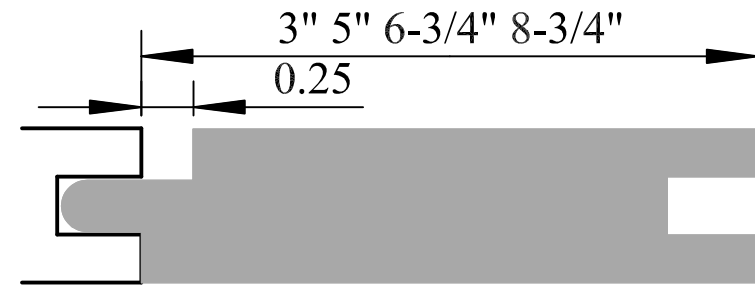
FL # 409 3/4" x 4"-10"
