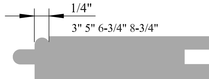
FL # 475 3/4"x 4"-10"
