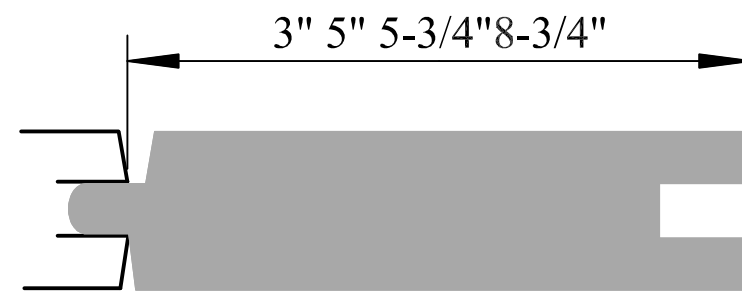
FL # 360 3/4"x 4"- 10"
