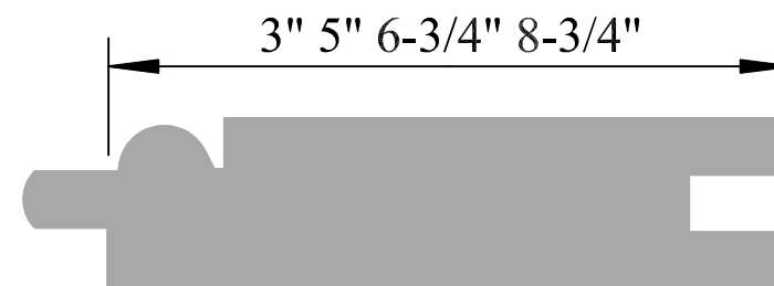
FL # 243 3/4"x 4"-10"
