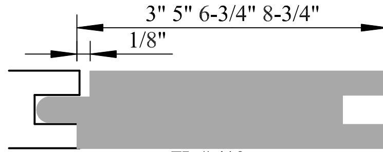
FL # 410 3/4"x 4"-10"
