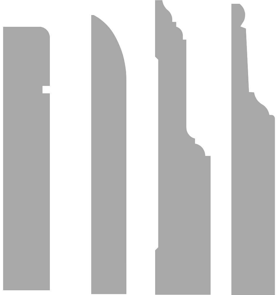
FL # 310 3/4"x 4-1/4"
