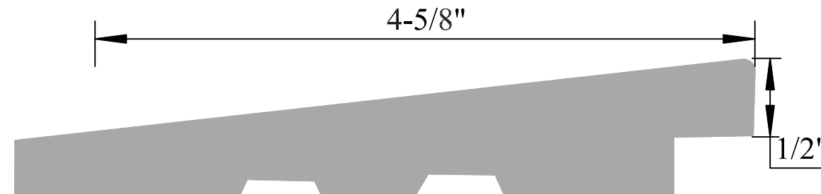
FL # 572 1"x 4-5/8"
