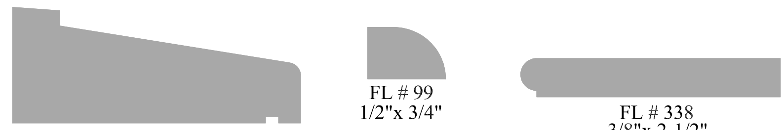
FL # 156 1" x 2-3/4"
