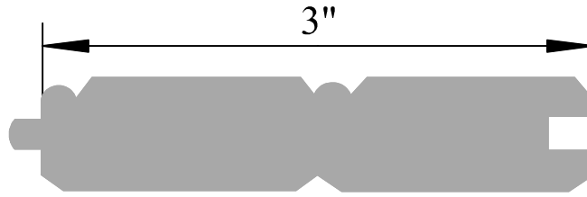
FL # 55 5/8"x 3"
