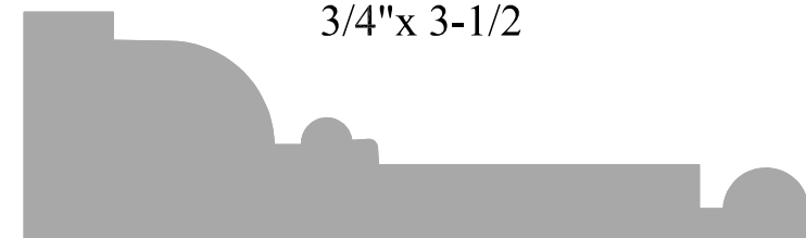
FL # 107 1" x 3-1/2"
