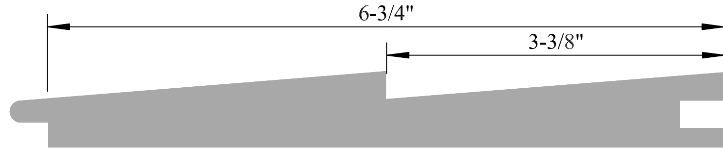
FL # 160 3/4"x 8"
