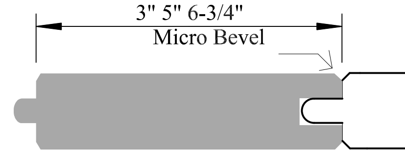
FL # 363 3/4"x 4"-8"
